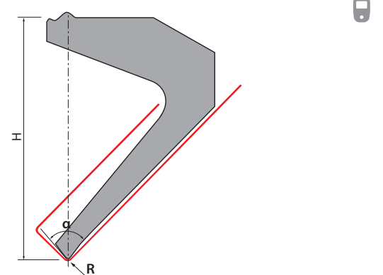
Front- and Hemming Tool (Foldings)
