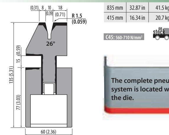
S135PN.26.10 1000 kN/m max.
