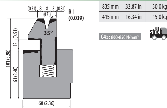
S101.35.08 600 kN/m max.
