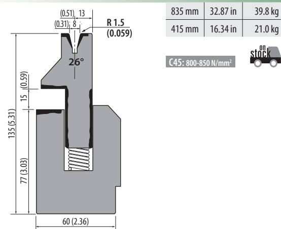
SA135.26.12 1000 kN/m max.
