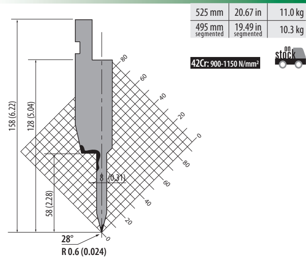
TOP.SP.134.28.8
