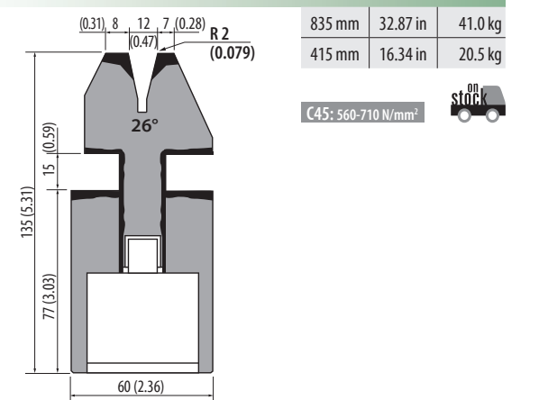
SA135PN.26.12 1000 kN/m max.
