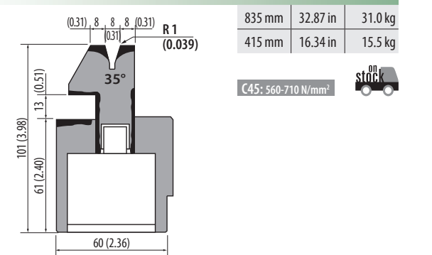
S101PN.35.08 600 kN/m max.
