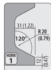
Horn 1 Standard for all segmented Punches Rolleri Type R2
