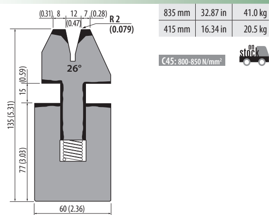
SA135.26.12 1000 kN/m max.
