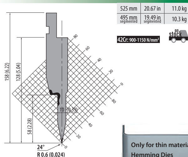
TOP.SP.134.24.10
