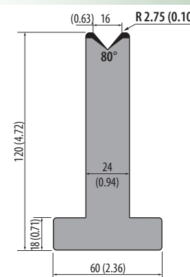
T120.16.80 950 kN/m max.
