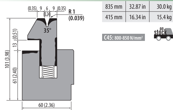
S101.35.06 600 kN/m max.
