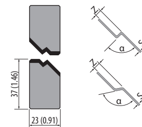
Z-Tool Inserts 160° / 150° / 140° / 90°
