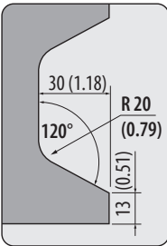
Standard-Horn Type for all segmented Punches Rolleri Type RX Gasparini
