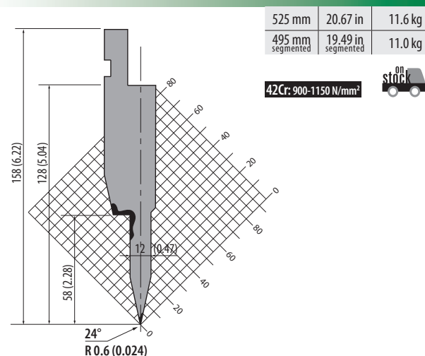
TOP.SP.134.24.12
