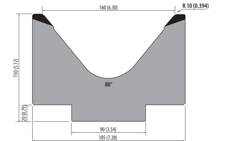
M130.80.160 1000 kN/m max.
