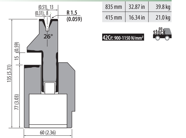
SA135PN.26.12 1000 kN/m max.
