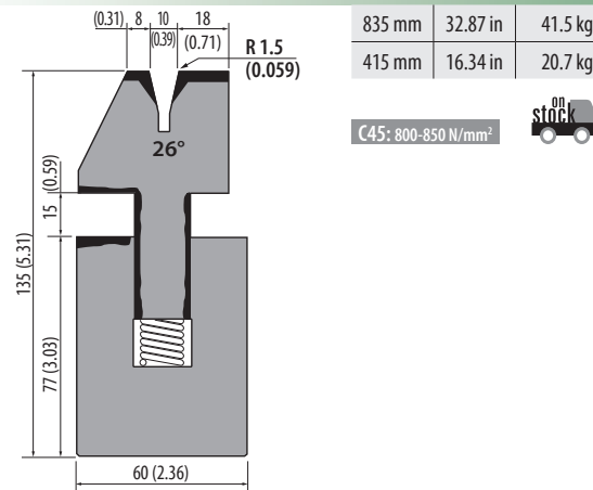
S135.26.10 1000 kN/m max.
