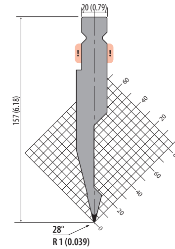
TPR157.28.R1
