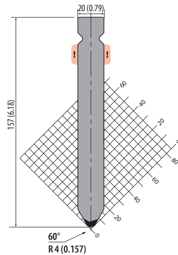
TPR157.60.R4
