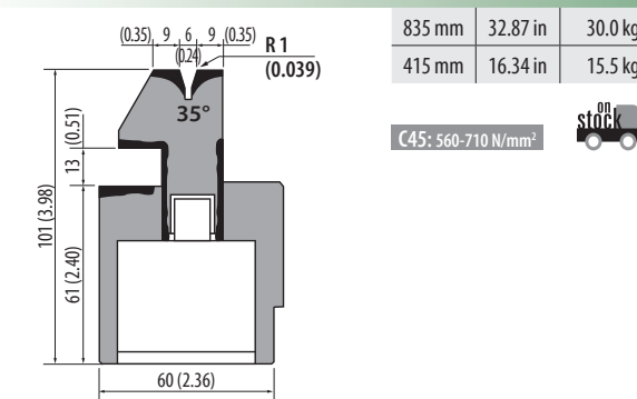
S101PN.35.06 600 kN/m max.
