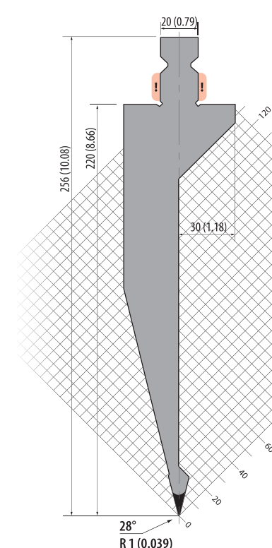
TPR256.28.R1
