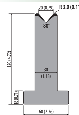
T120.20.80 950 kN/m max.
