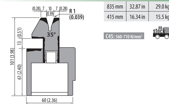
S101PN.35.10 600 kN/m max.
