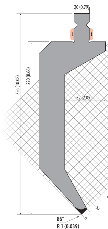
TPR256.86.R1
