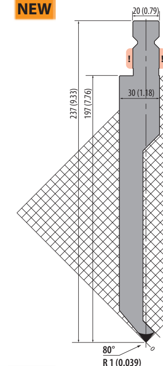
TPR237.80.R1
