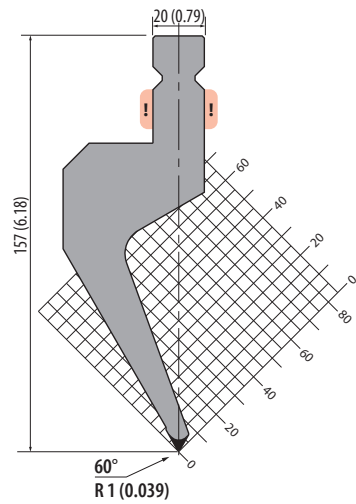
TPR157.60.R1
