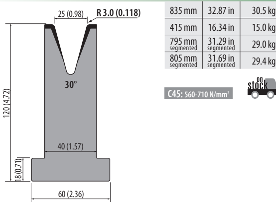
T120.25.30 500 kN/m max.
