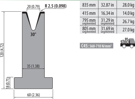
T120.20.30 500 kN/m max.
