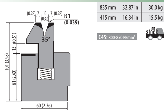
S101.35.10 600 kN/m max.
