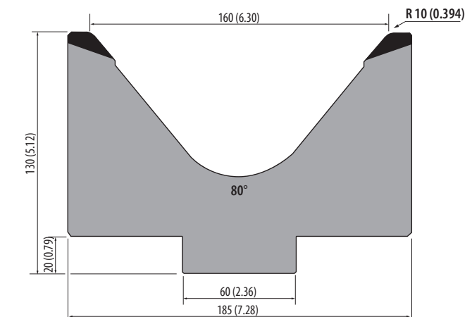
MK130.80.160 700 kN/m max.
