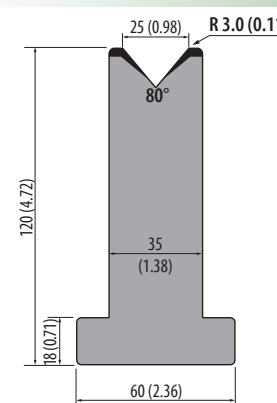
T120.25.80 950 kN/m max.
