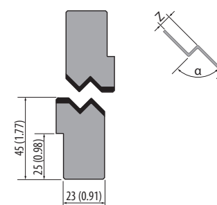
Z-Tool Inserts 90°
