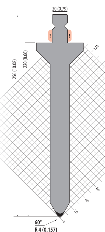
TPR256.60.R4
