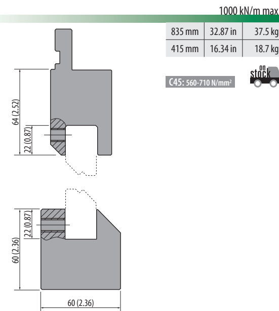
Z-Tool Inserts 160° / 150° / 140° / 90°
