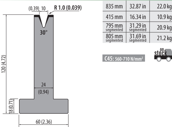
T120.16.30 450 kN/m max.
